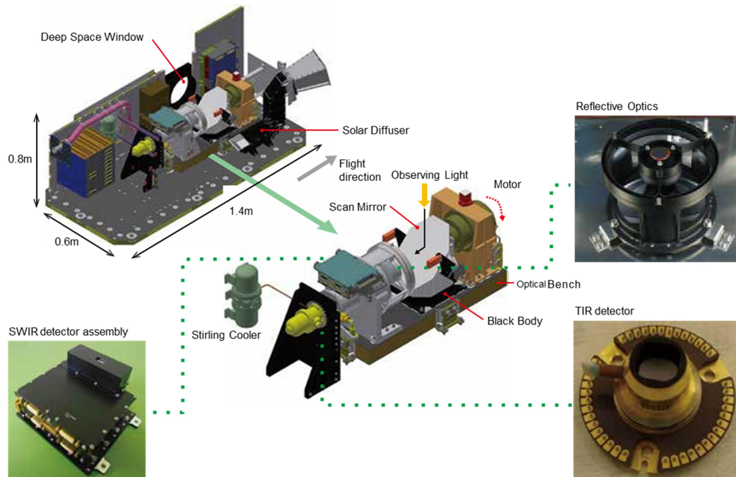
Figure 2-9 IRS SRU
