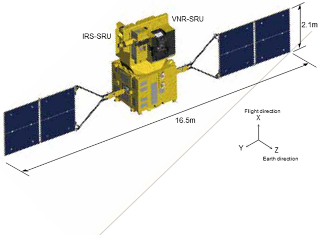
Figure 2-1 Appearance of GCOM-C
