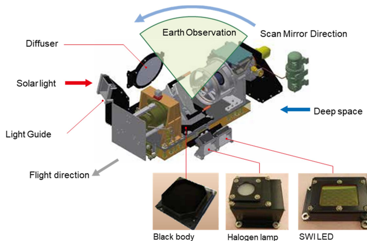
Figure 2-14 IRS Calibration Features
