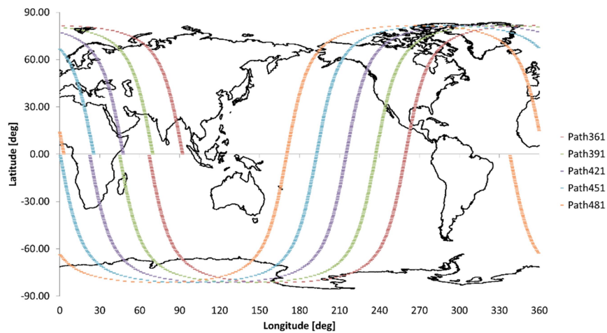
Figure 4-5 GCOT-C Path Definition (Path361 to 481)
