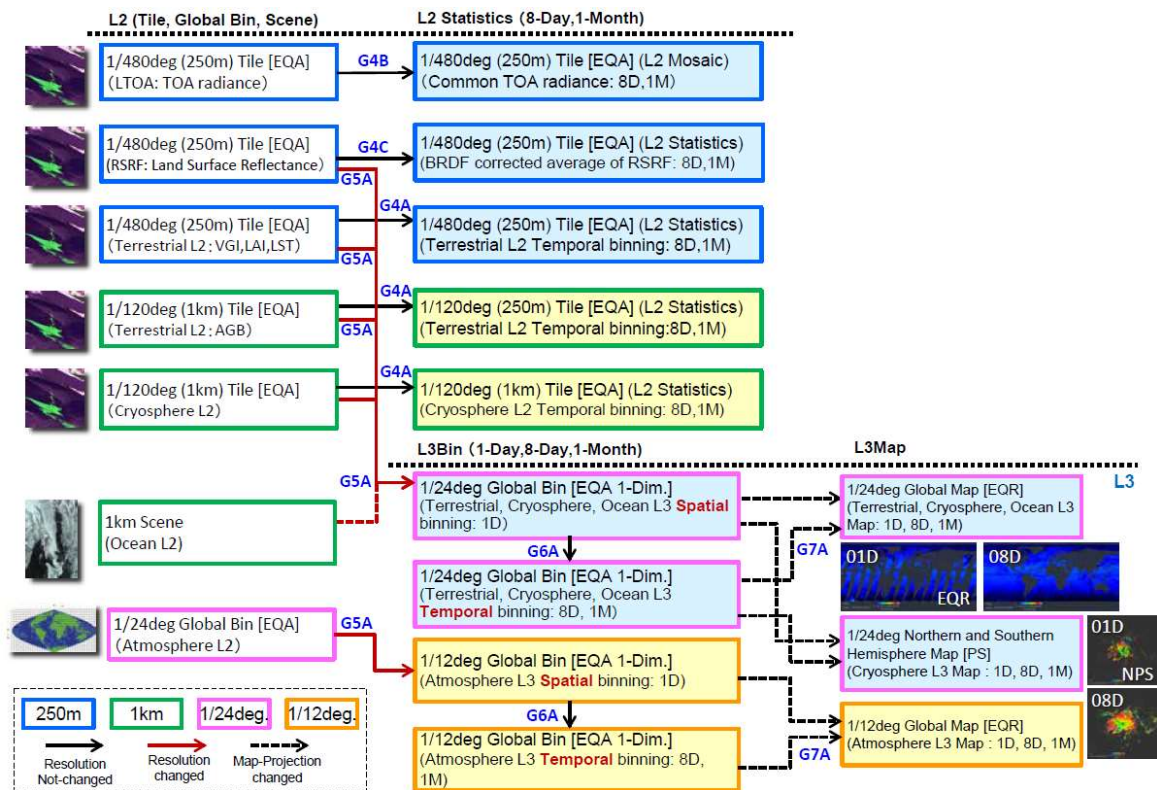
Figure 4-2 SGLI Level2 and Level3 Processing Flow
