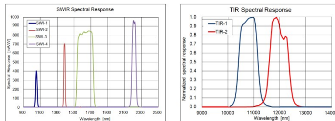
Figure 2-5 IRS Response Function
