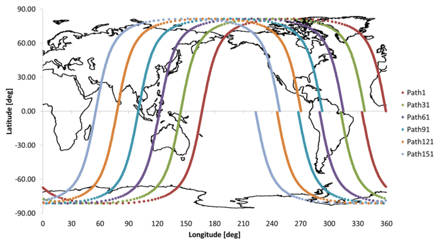
Figure 4-3 GCOT-C Path Definition (Path 1 to 151)
