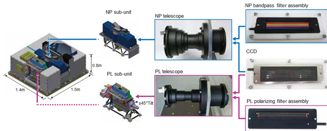
Figure 2-8 VNR SRU
