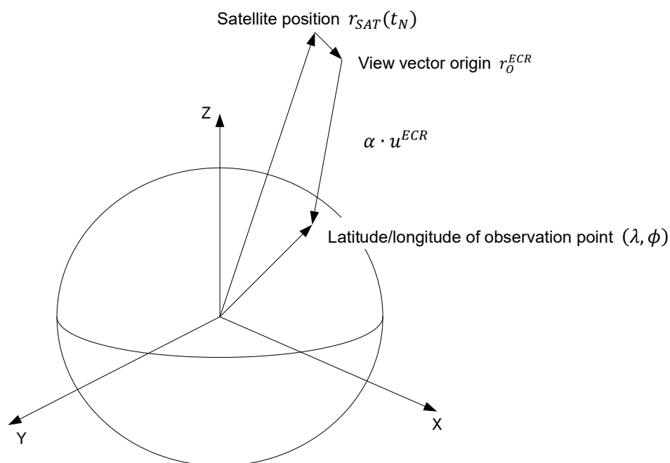
Figure 4-17 Schematic Diagram: Calculation of Latitude/longitude of Observation Point
