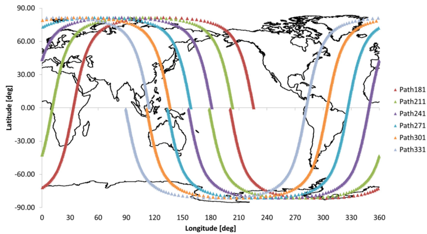
Figure 4-4 GCOT-C Path Definition (Path 181 to 331)
