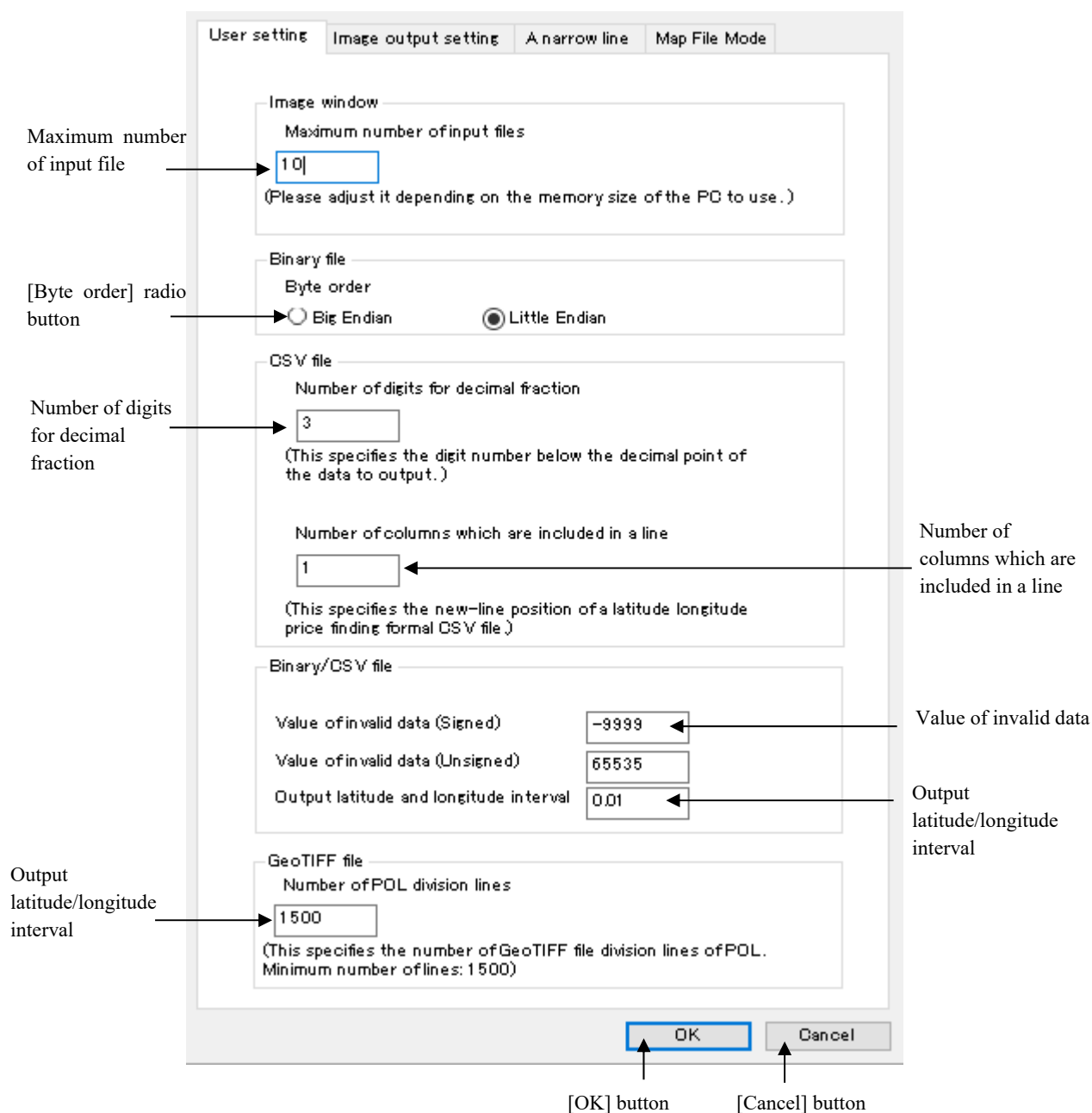
Figure 4.3.3-1 Image of User Setting Dialog
